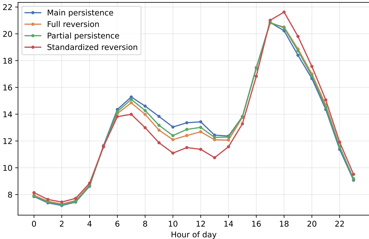
Stock-weighted whole-building load (kW)
